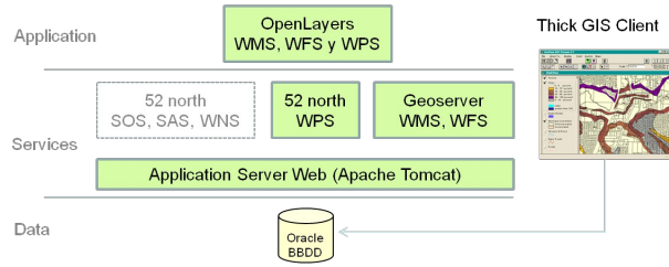
Figure 11. Implemented service and application architecture
